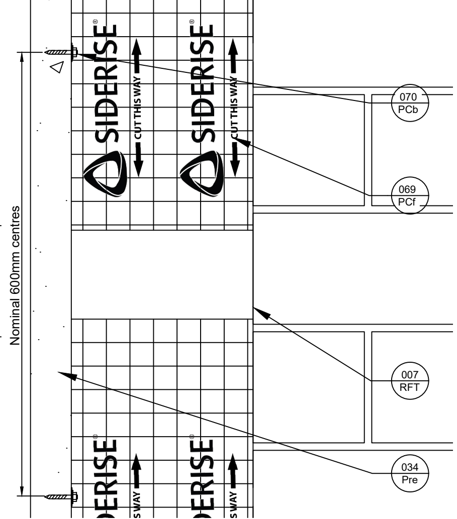
Side View
