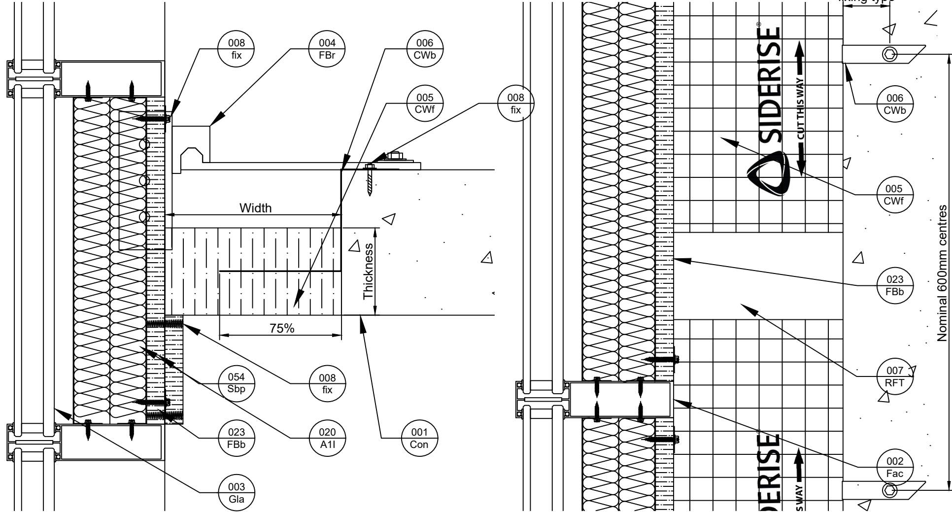
Plan View (Below Firestop)
