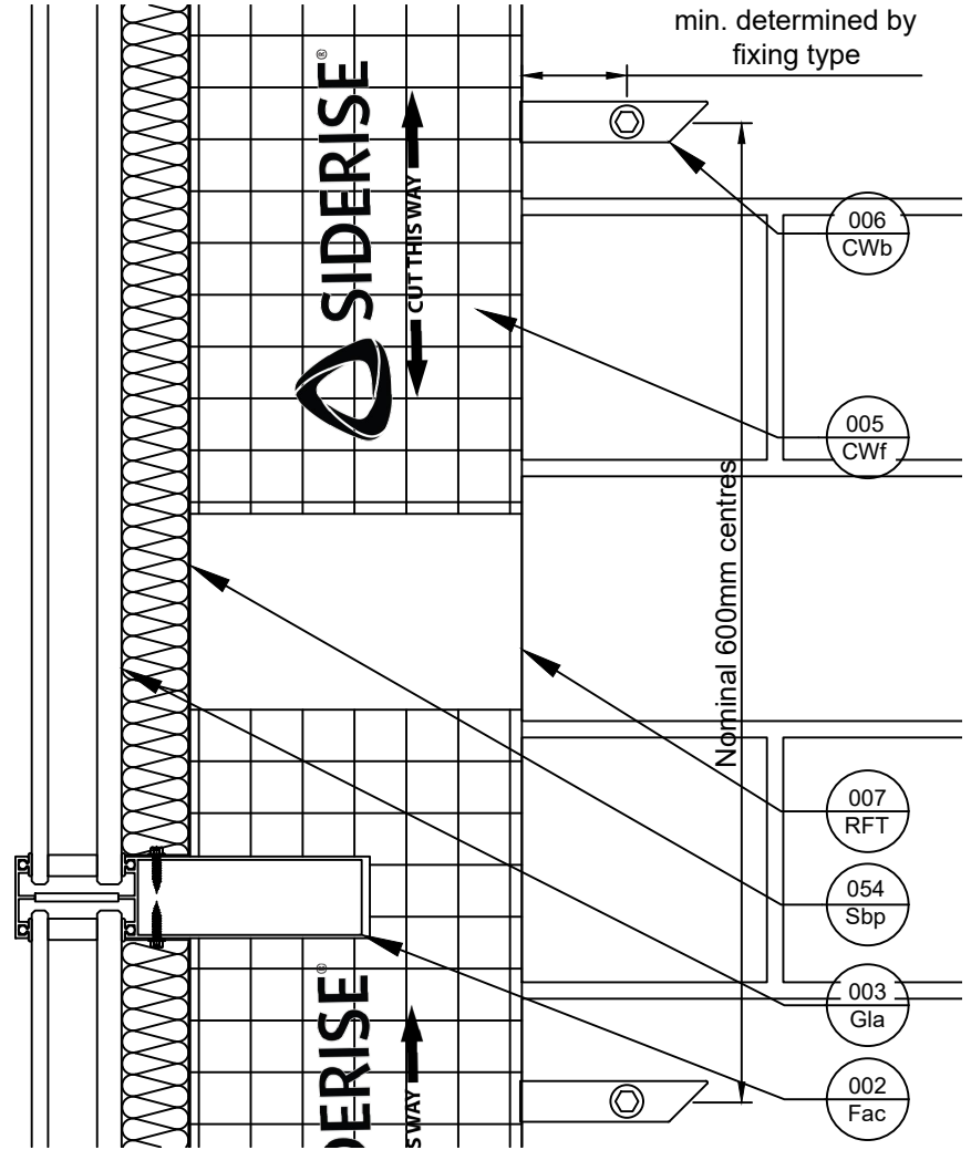
Side View
