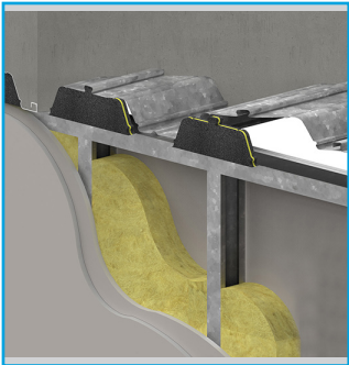
Fig 1. Profiled deck/Top of Wall junc.
