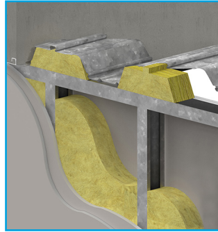
Fig 3. SIDERISE TW-PP installed
