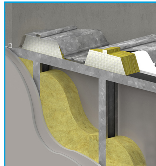
Fig 4. SIDERISE TW-PS installed
