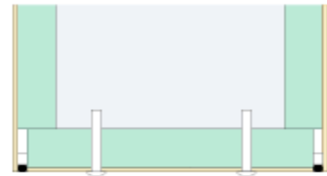
Sealed external corner joint
