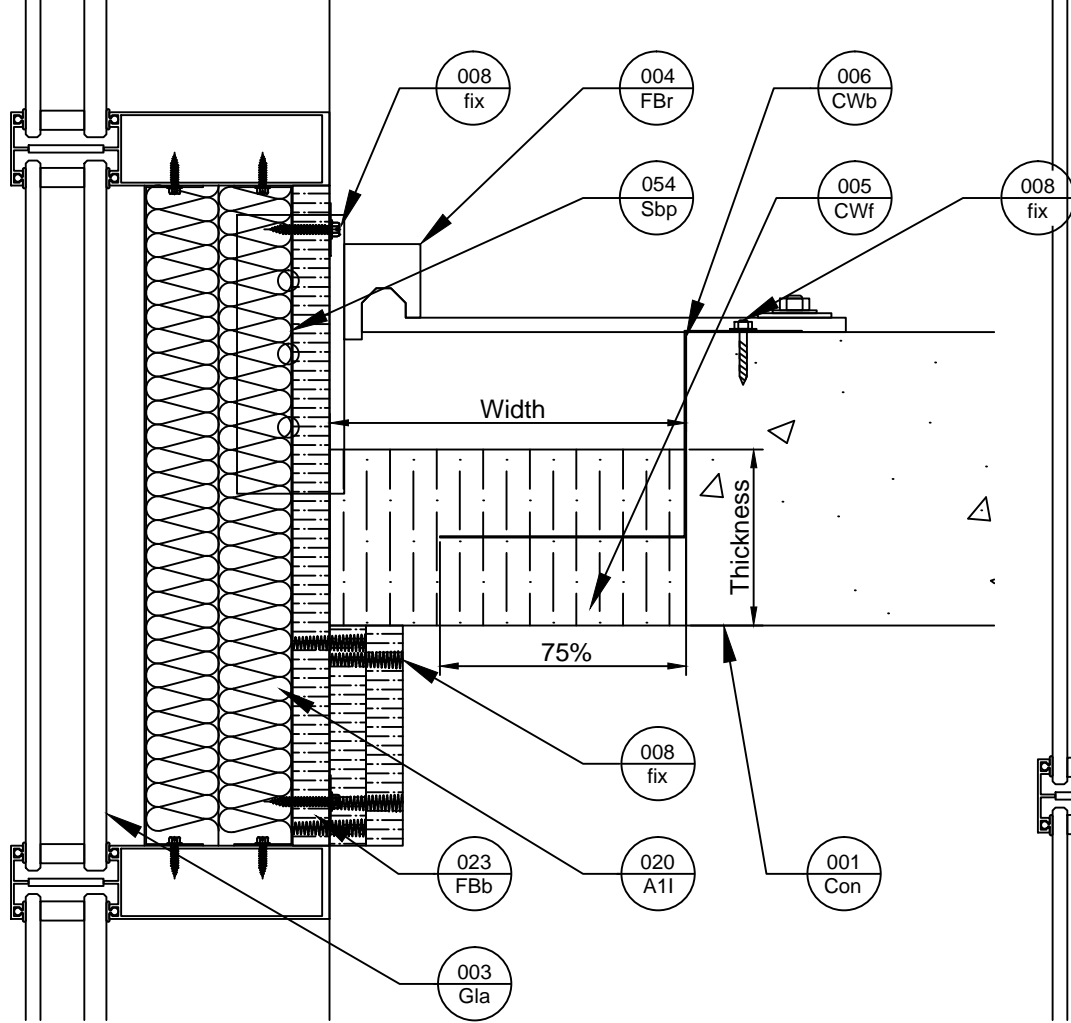
Plan View (Below Firestop)
