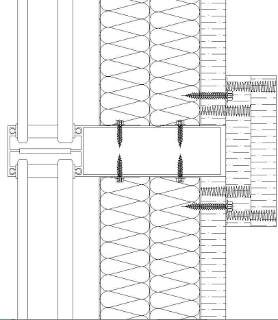
Plan View (Below Firestop)
