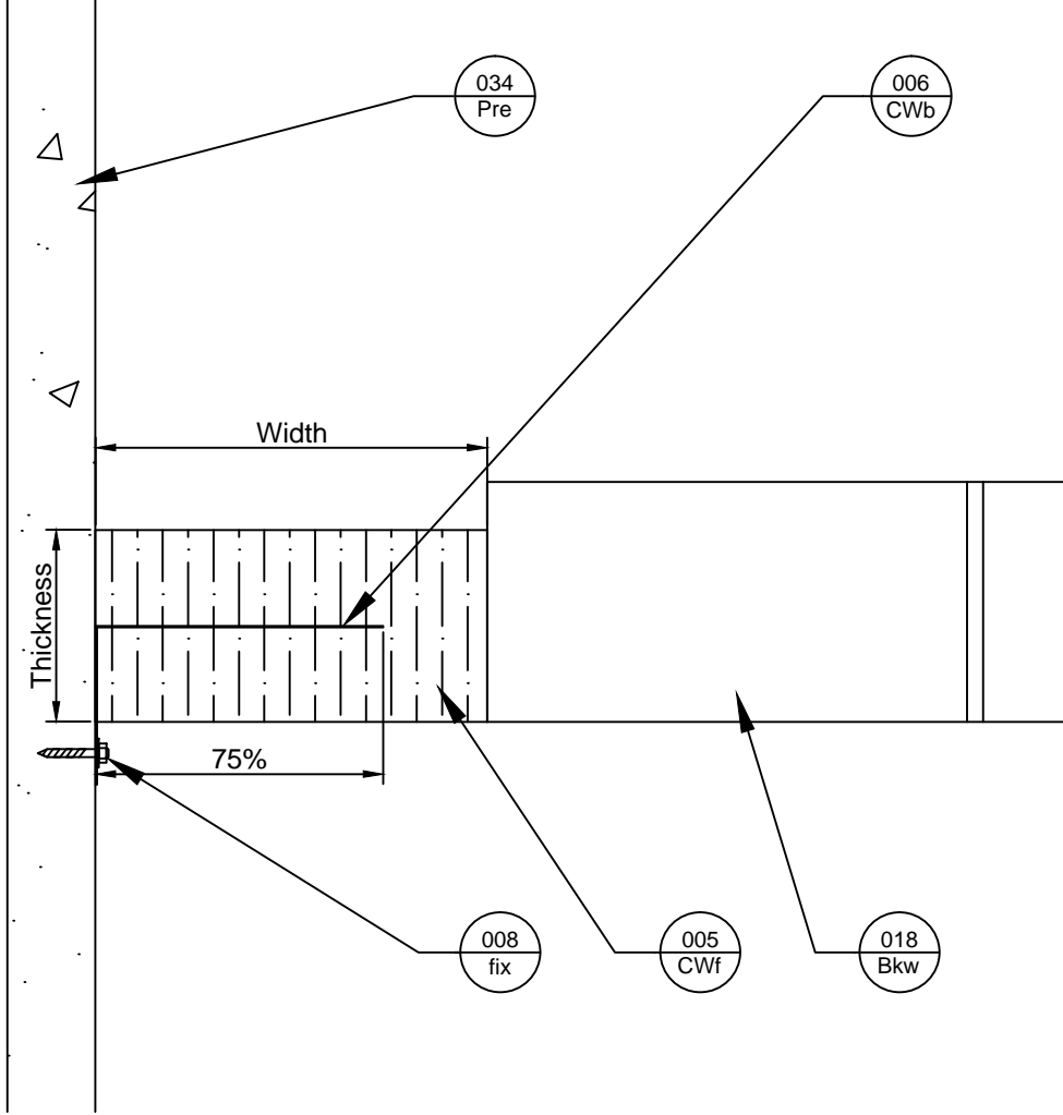
Plan View
