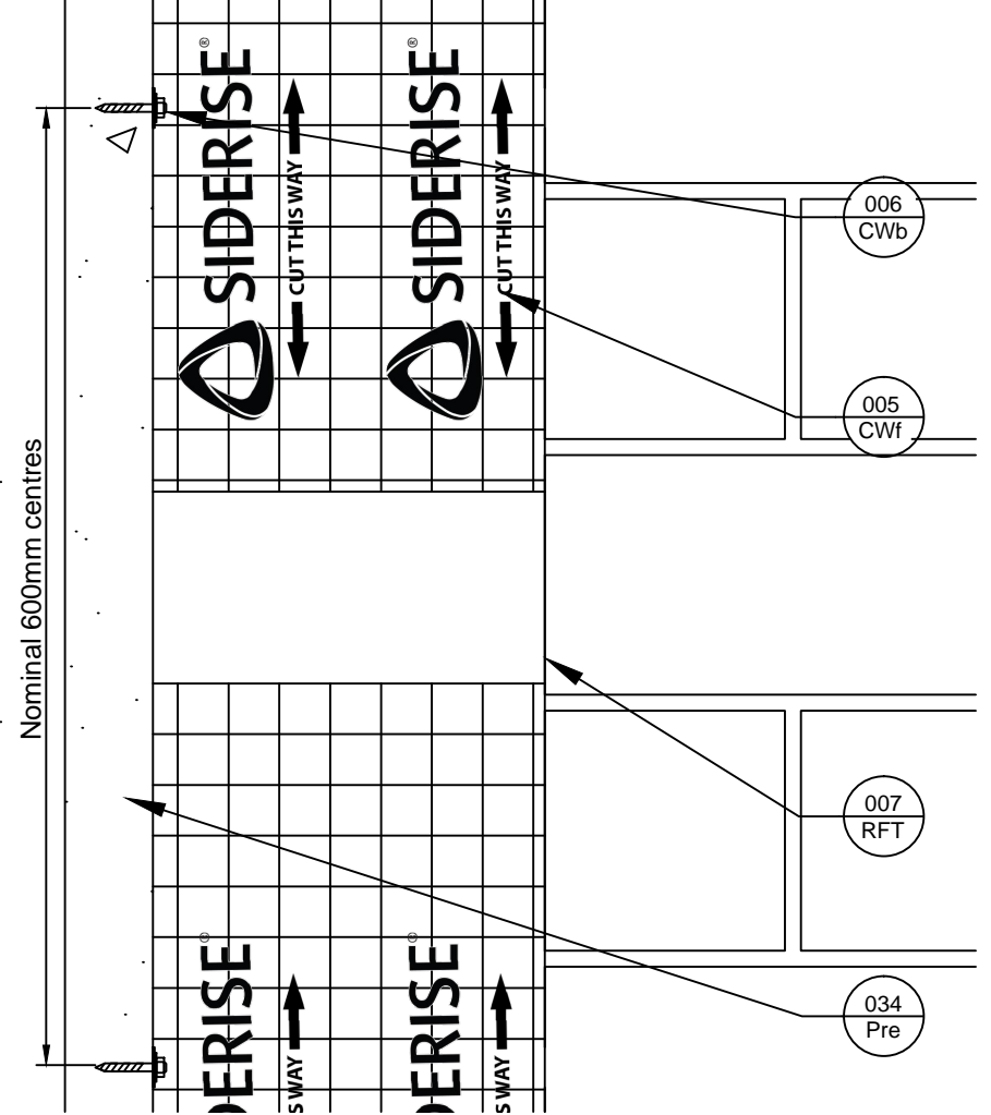
Side View
