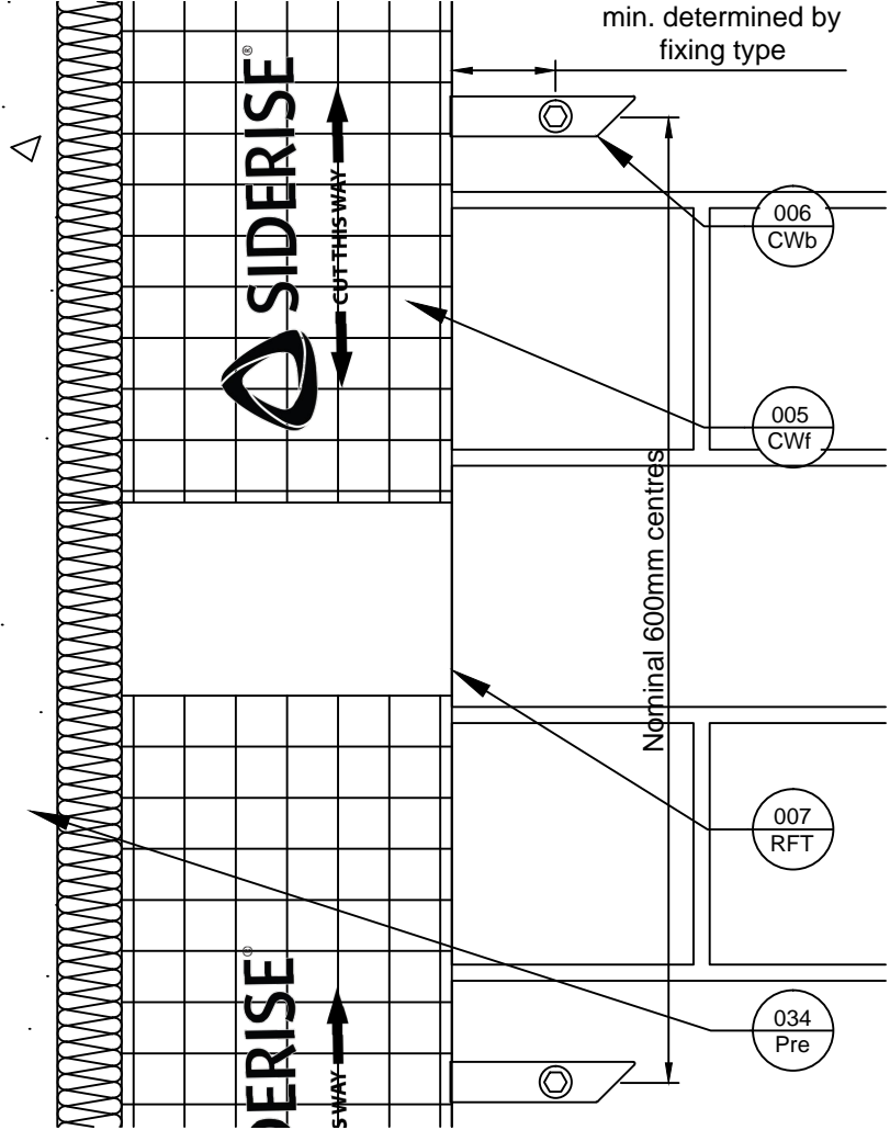
Side View
