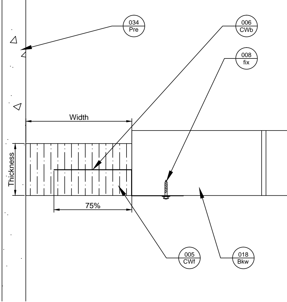
Plan View
