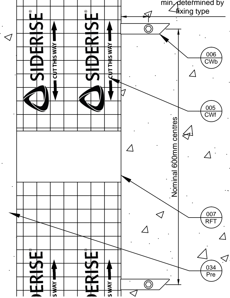
Plan View
