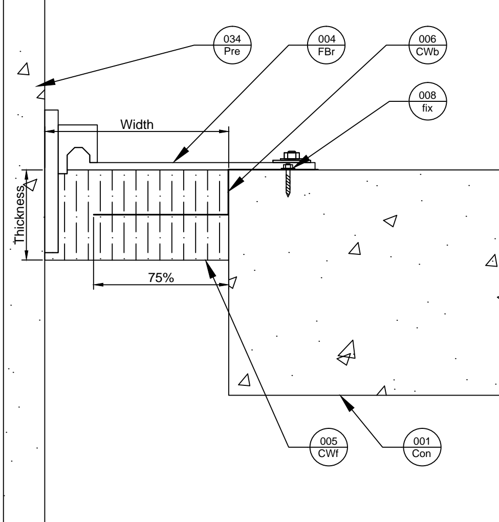
Side View
