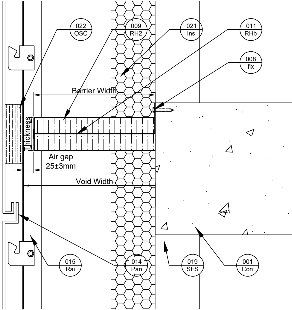
Side View
