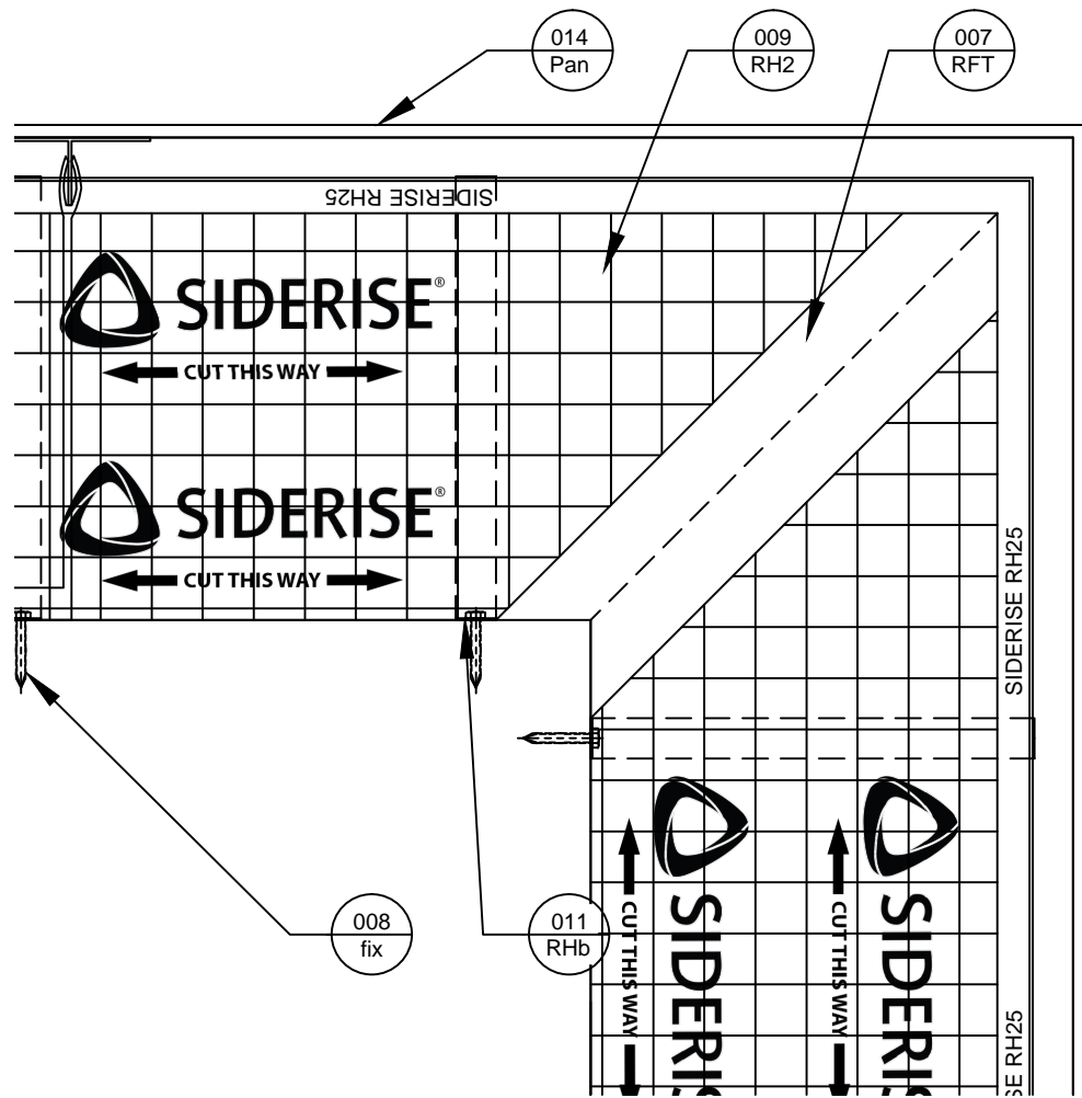
Plan View
