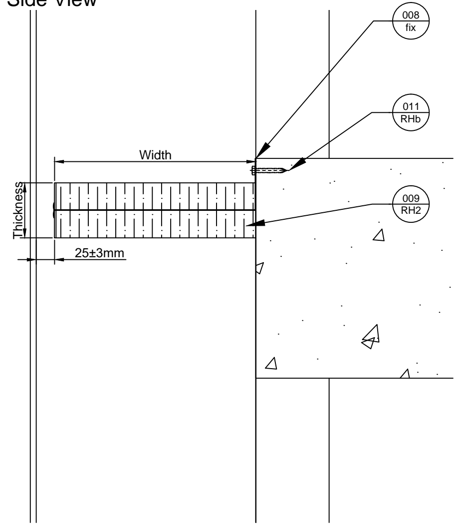
Side View
